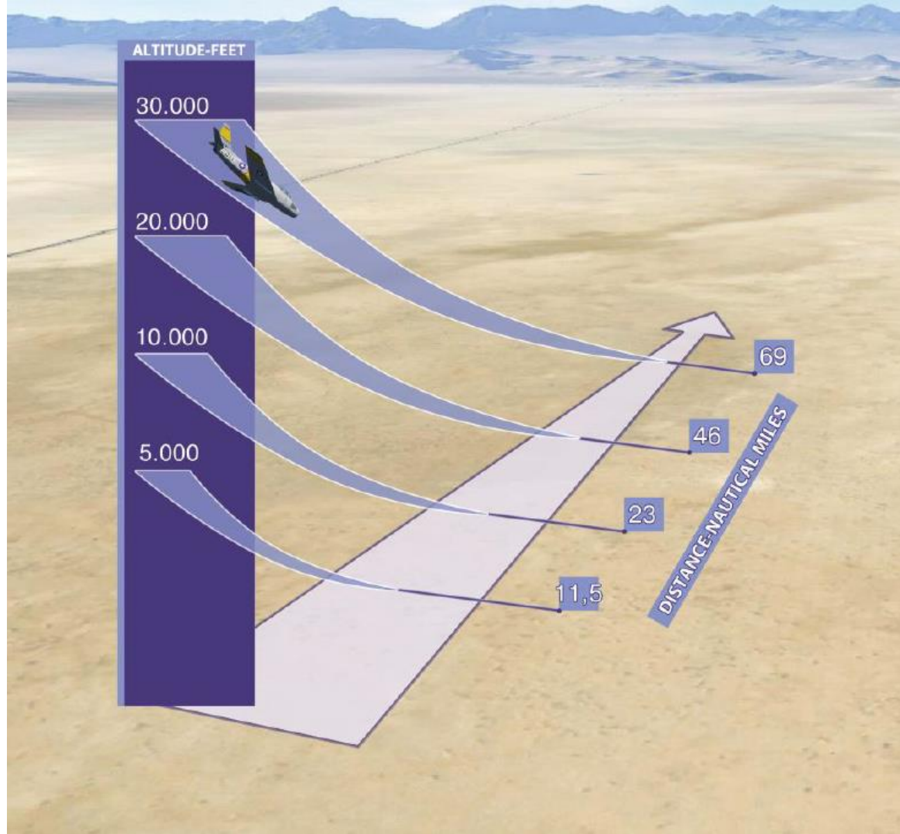
Gliding distances (nm) from different altitudes (ft) with the engine off
