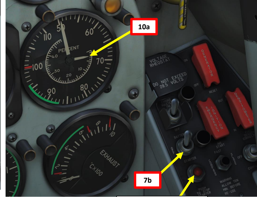
Stop-Starter Button
