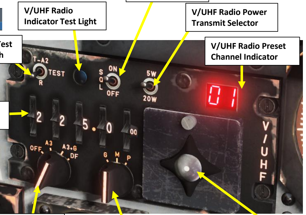
V/UHF Radio Squelch Switch
