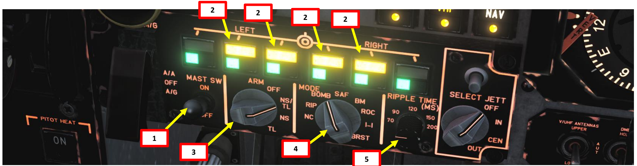
Figure 9-40 Pylon Selector/Status Indicator Buttons
