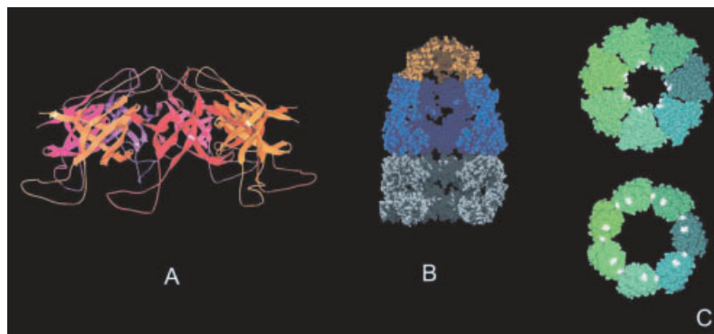
Figure 13.6 Structure of the GroEL chaperonin from E. coli . (A) Sideview of the GroES heptamer. The individual subunits (in shades of red) consist mainly of \beta -sheets and form a dome. The flexible extensions on the bottom are the so-called mobile loops that mediate binding to GroEL. (B) Cross-section of a GroE “bullet”. Each GroEL ring encloses a cavity that serves as a folding compartment for a polypeptide substrate. Binding of GroES (orange) to the top GroEL ring (blue) blocks the access to the upper cavity and concomitantly induces an en bloc movement of the apical domains. (C) Changes in the GroEL structure upon binding of GroES. In this top view, the seven subunits comprising one ring of GroEL are shown in shades of green and blue. The hydrophobic residues in the apical domains important for binding of polypeptide and GroES are shown in white. In the absence of GroES (top panel), these residues coat the inside of the central cavity and account for the high affinity for unfolded polypeptides. Upon binding of GroES (lower panel) the apical domains rotate outwards by 90°. The hydrophobic patches become buried in the subunit interfaces, rendering the inner surface of the cavity mainly hydrophilic and causing the release of a bound polypeptide. Concomitantly, the diameter of the cavity increases from 45 to 80 Å. Reprinted with permission from Walter [71].
