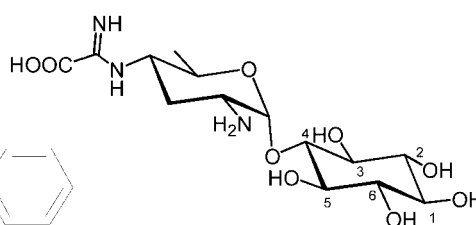
Kasugamycin
