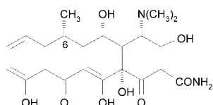
Doxycycline (6-deoxy-tetracycline) (1967)
