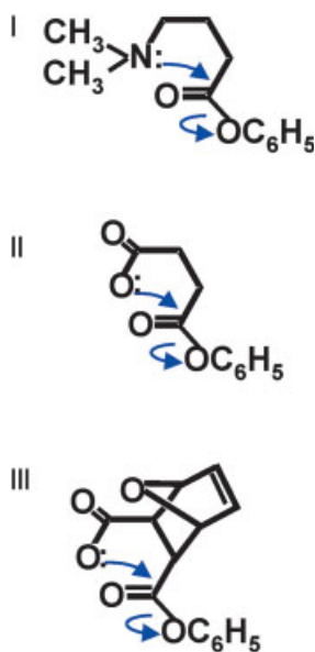
Figure 8-11 Peptide-bond formation in model compounds with appropriate juxtaposed nucleophile. See text for explanations.
