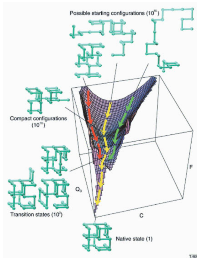
Figure 13.1 Free-energy landscape of the fold-ing of a protein. The free energy (F) surface or free energy landscape of a protein is repres-ented as a function of the number of native contacts (Q) and the total number of (native and nonnative) contacts (C). Native and non-native contacts refer to contacts bringing or not towards the native state, respectively. The surface shown in the figure illustrates that at the beginning of the folding reaction there are many conformations of similar free energy, so that the accessible surface is very broad. As folding progresses, the energy of the system decreases with the formation of native contacts that are generally
