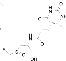
Sparsomycin
