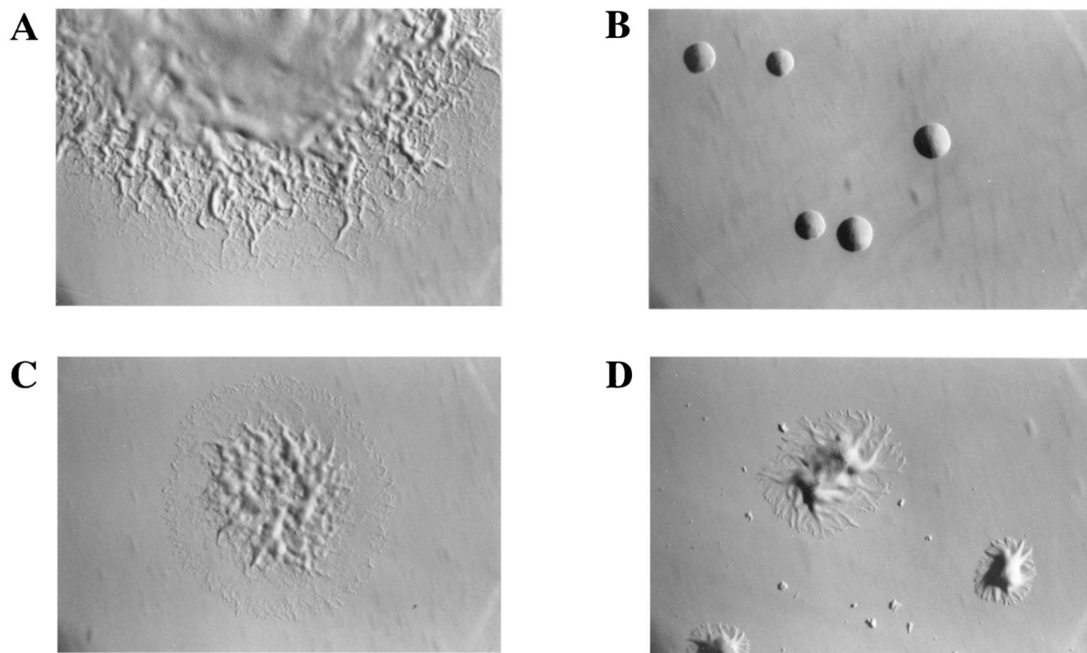
FIG. 4. Photomicrographs of F. johnsoniae colonies. Colonies were grown for 2 days at 25°C on PY2 agar medium. Photomicrographs were taken with an Olympus OM-4T camera mounted on a Nikon Diaphot inverted phase-contrast microscope. (A) Wild-type F. johnsoniae UW101. (B) gldBC knockout mutant CJ588. (C) CJ594 (CJ588 complemented with pDH233, which carries gldBC ). (D) CJ767 (CJ588 complemented with pDH246, which carries gldB ). Bar, 1 mm.
