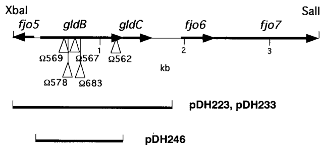
FIG. 2. Map of the gldB region. The sites of the Tn4351 insertions in CJ562, CJ567, CJ569, CJ578, and CJ683 are indicated by triangles. Regions of F. johnsoniae DNA contained in pDH223, pDH233, and pDH246 are shown beneath the map.
